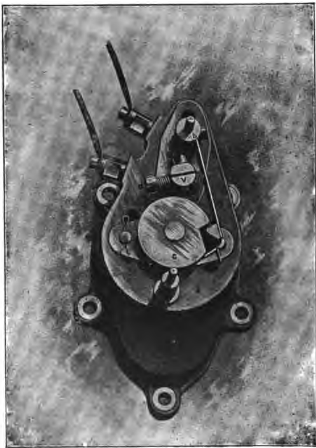
FIG. 333.—The De Dion Circuit Breaker. The parts lettered are the same as those indicated in Fig. 332.
